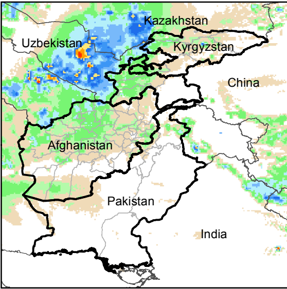
Daily Rainfall estimate for 30 Mar., 2016
