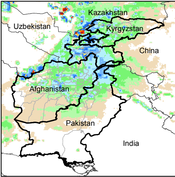
Daily Rainfall estimate for 31 Mar., 2016
