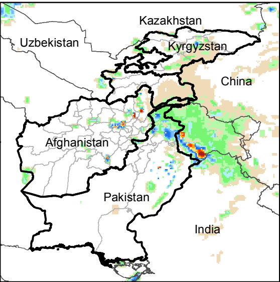
Daily Rainfall estimate for 29 Mar., 2016
