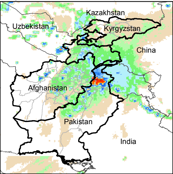
Daily Rainfall estimate for 6 Apr., 2016
