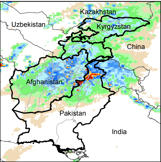
Daily Rainfall estimate for 5 Apr., 2016
