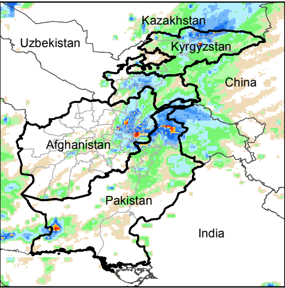
Daily Rainfall estimate for 9 Apr., 2016
