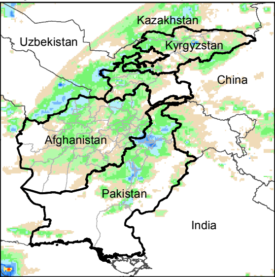
Daily Rainfall estimate for 11 Apr., 2016
