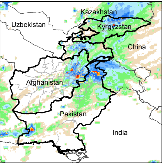
Daily Rainfall estimate for 12 Apr., 2016
