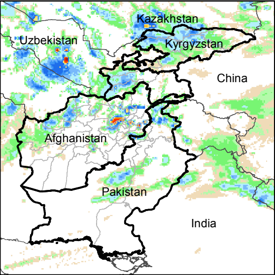
Daily Rainfall estimate for 21 Apr., 2016
