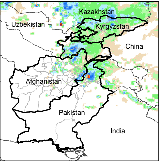
Daily Rainfall estimate for 24 Apr., 2016
