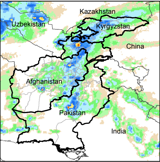
Daily Rainfall estimate for 3 May., 2016
