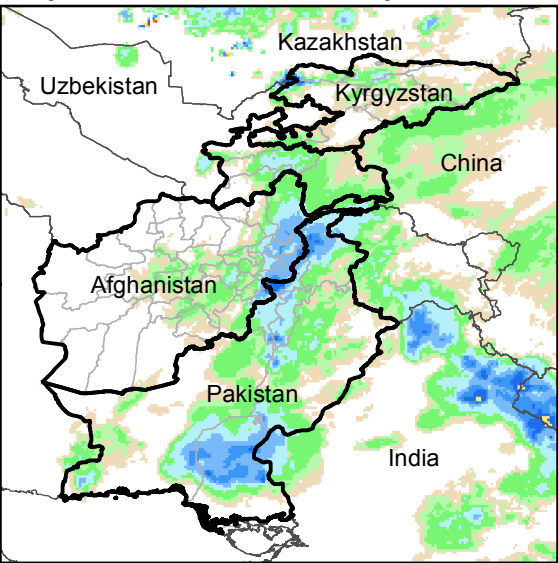
Daily Rainfall estimate for 4 May., 2016
