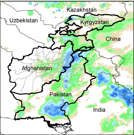
Daily Rainfall estimate for 7 May., 2016
