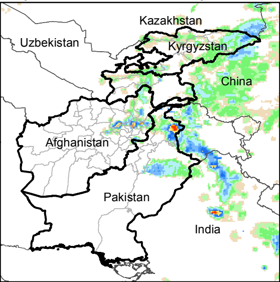
Daily Rainfall estimate for 27 May., 2016
