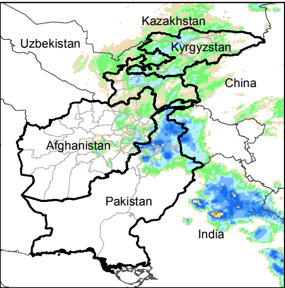
Daily Rainfall estimate for 26 May., 2016
