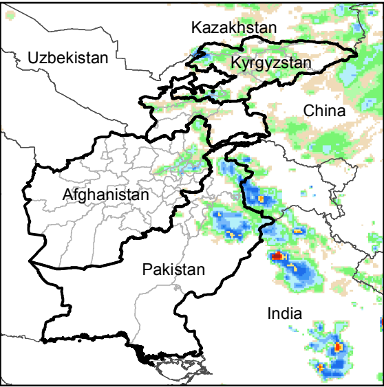
Daily Rainfall estimate for 30 May., 2016
