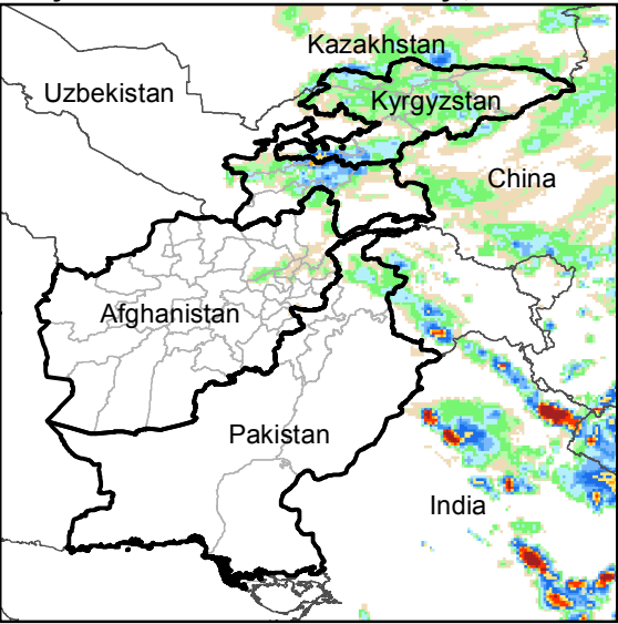
Daily Rainfall estimate for 29 May., 2016
