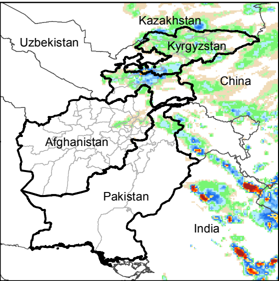
Daily Rainfall estimate for 1 Jun., 2016
