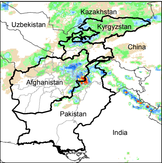
Daily Rainfall estimate for 6 Jun., 2016
