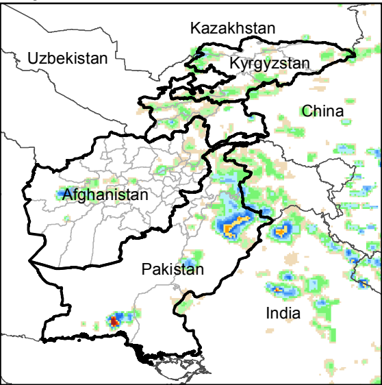
Daily Rainfall estimate for 13 Jun., 2016
