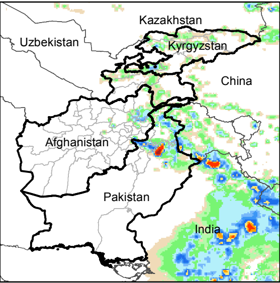
Daily Rainfall estimate for 20 Jun., 2016
