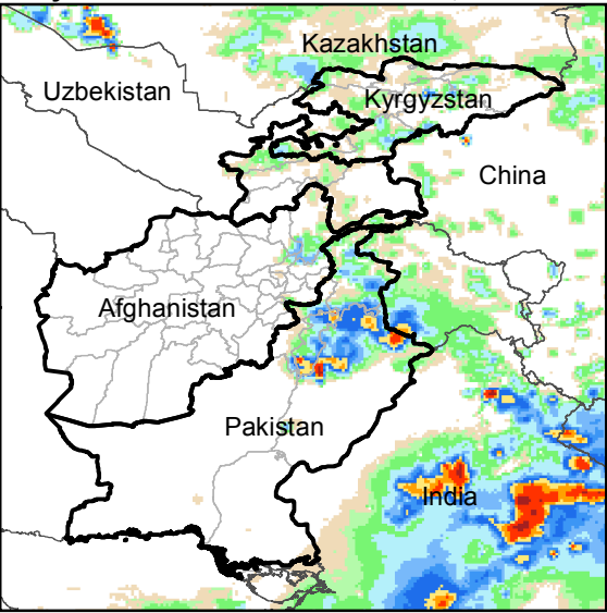
Daily Rainfall estimate for 21 Jun., 2016
