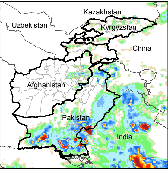
Daily Rainfall estimate for 28 Jun., 2016
