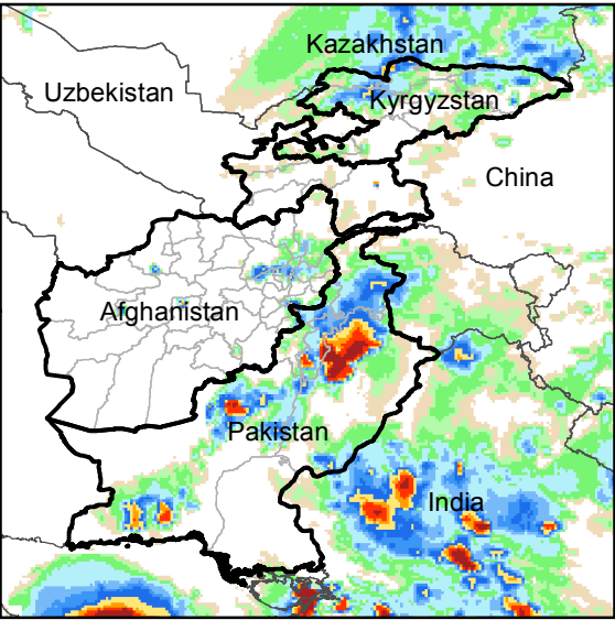
Daily Rainfall estimate for 27 Jun., 2016
