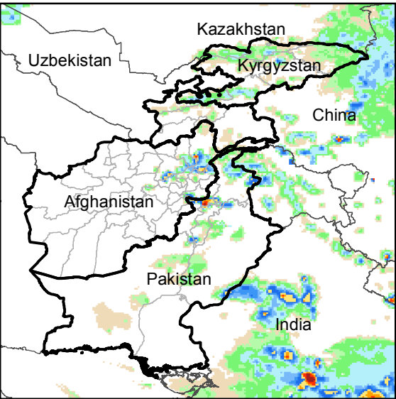
Daily Rainfall estimate for 26 Jun., 2016
