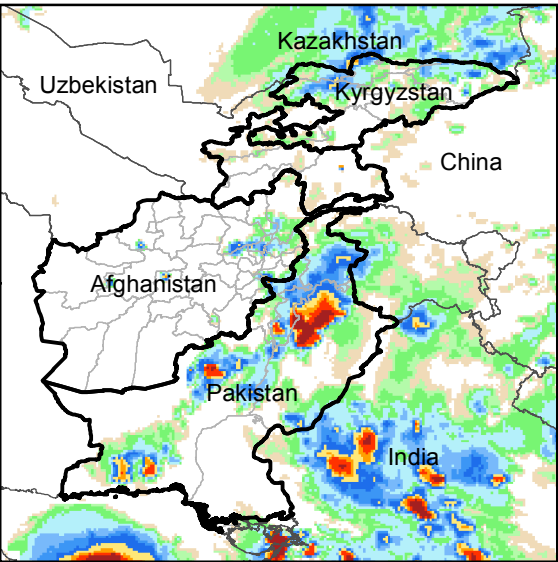
Daily Rainfall estimate for 30 Jun., 2016
