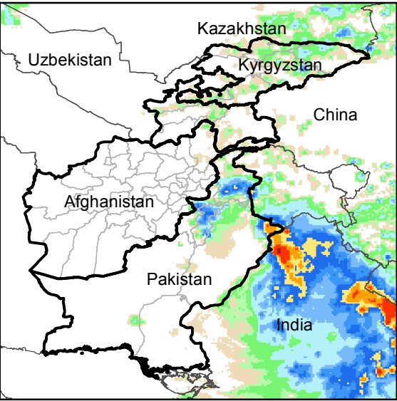
Daily Rainfall estimate for 2 Jul., 2016
