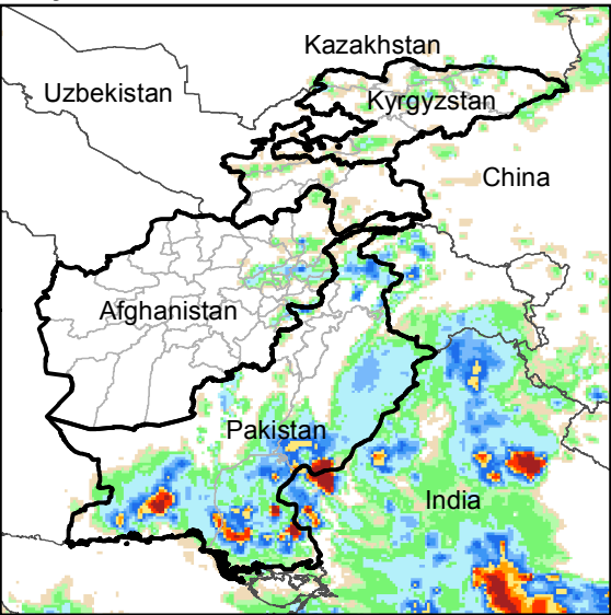
Daily Rainfall estimate for 1 Jul., 2016
