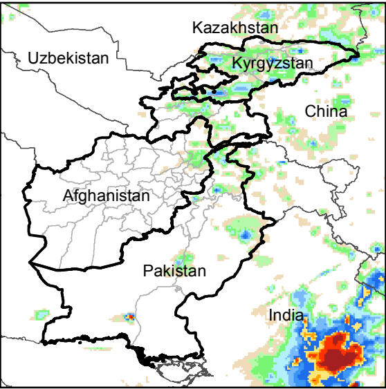
Daily Rainfall estimate for 7 Jul., 2016
