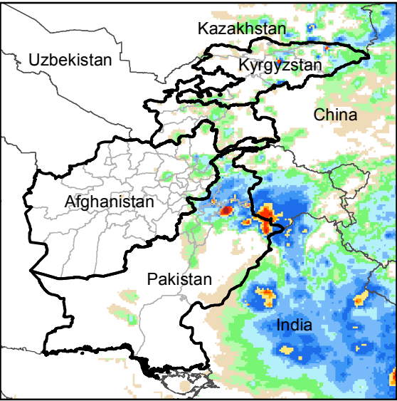
Daily Rainfall estimate for 15 Jul., 2016
