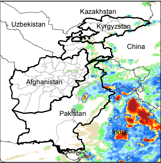
Daily Rainfall estimate for 16 Jul., 2016
