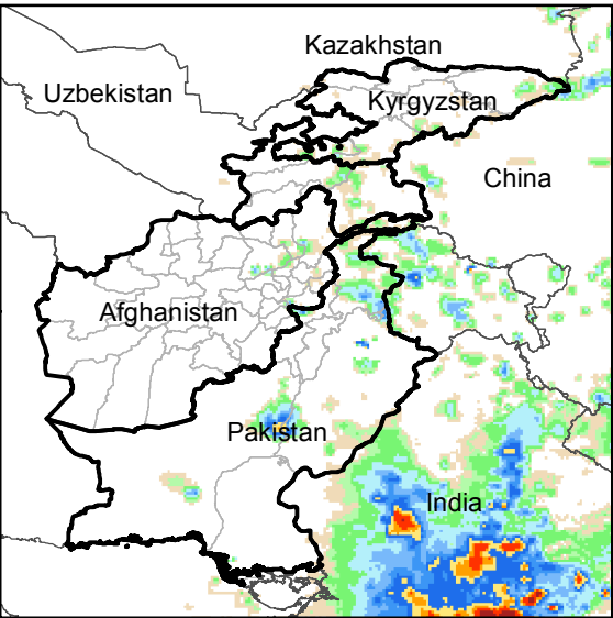
Daily Rainfall estimate for 14 Jul., 2016
