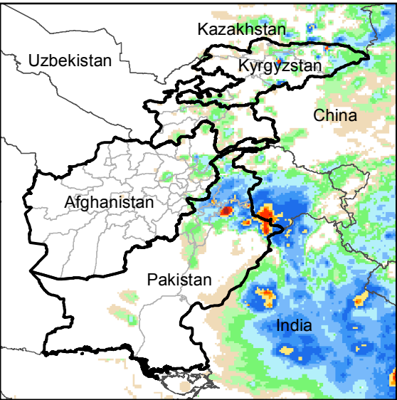
Daily Rainfall estimate for 18 Jul., 2016
