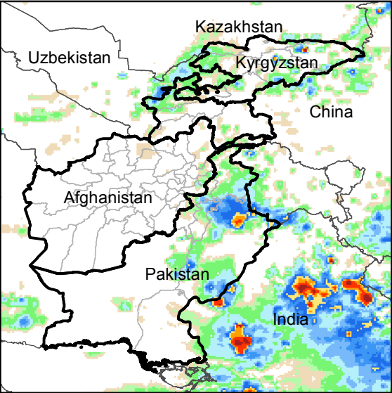
Daily Rainfall estimate for 30 Jul., 2016
