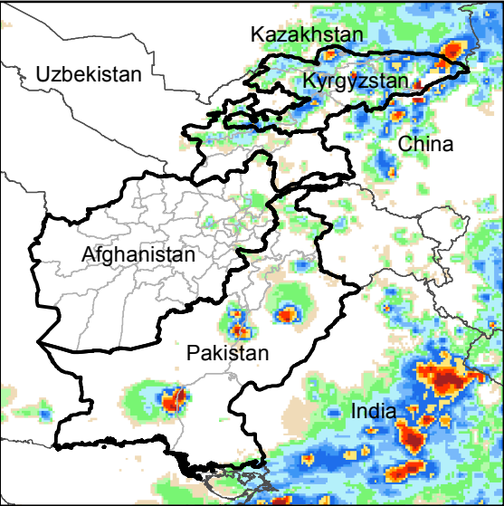
Daily Rainfall estimate for 31 Jul., 2016
