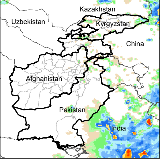
Daily Rainfall estimate for 1 Aug., 2016
