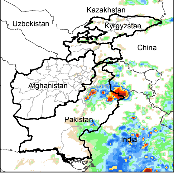
Daily Rainfall estimate for 2 Aug., 2016
