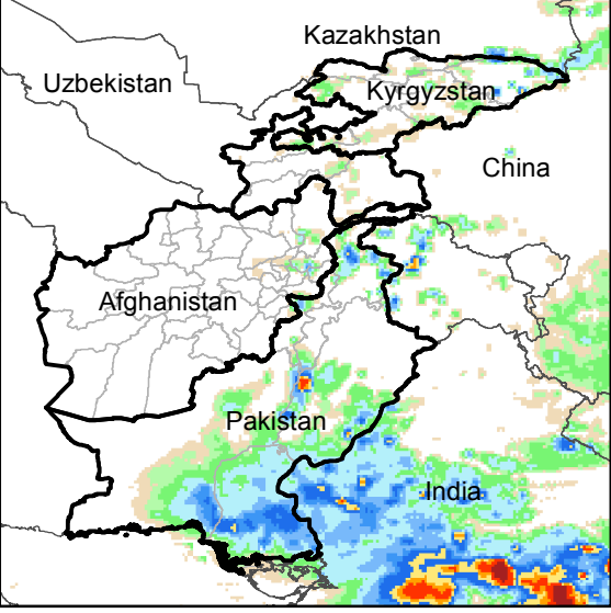
Daily Rainfall estimate for 3 Aug., 2016
