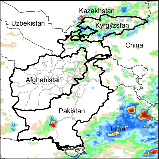
Daily Rainfall estimate for 29 Jul., 2016
