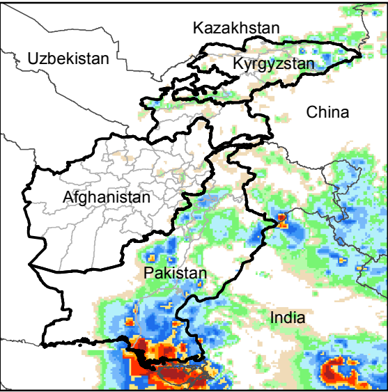
Daily Rainfall estimate for 5 Aug., 2016
