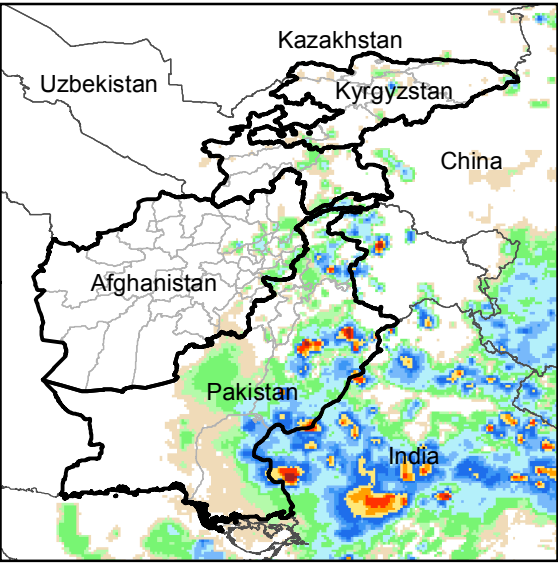
Daily Rainfall estimate for 8 Aug., 2016
