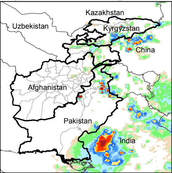
Daily Rainfall estimate for 12 Aug., 2016
