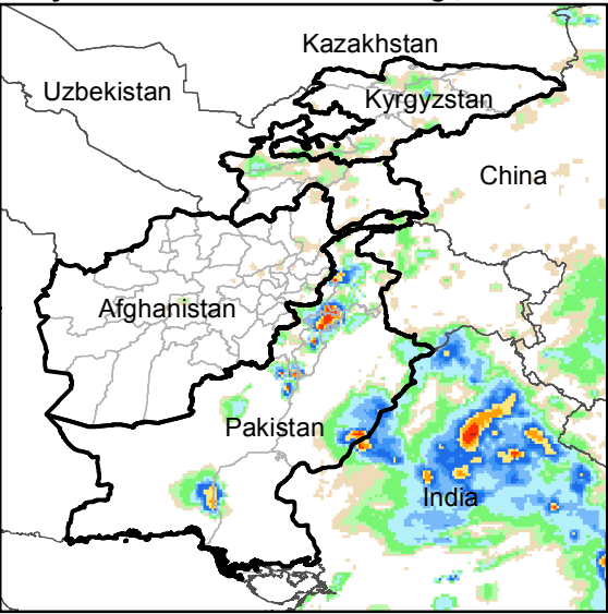
Daily Rainfall estimate for 11 Aug., 2016
