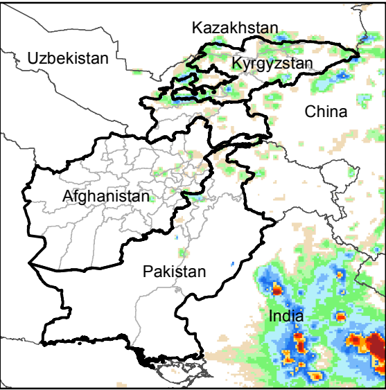
Daily Rainfall estimate for 13 Aug., 2016
