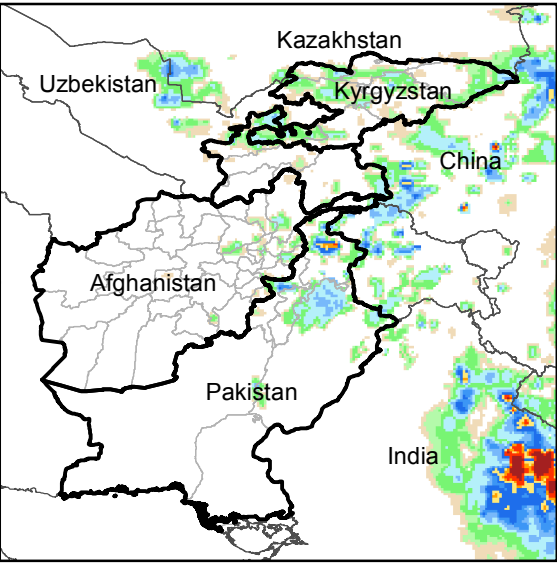
Daily Rainfall estimate for 15 Aug., 2016
