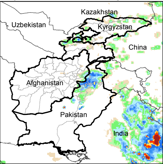
Daily Rainfall estimate for 17 Aug., 2016
