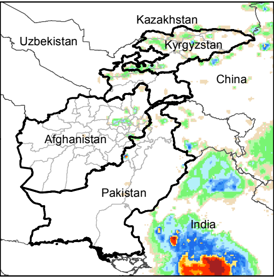
Daily Rainfall estimate for 20 Aug., 2016
