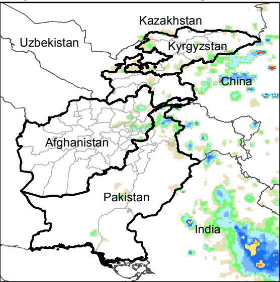
Daily Rainfall estimate for 21 Aug., 2016
