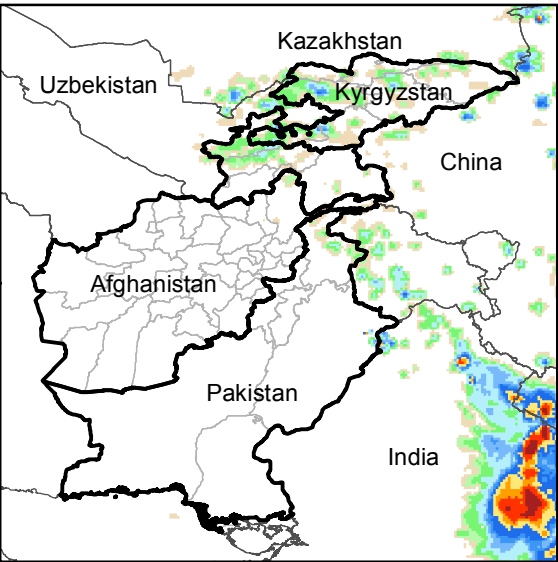
Daily Rainfall estimate for 19 Aug., 2016
