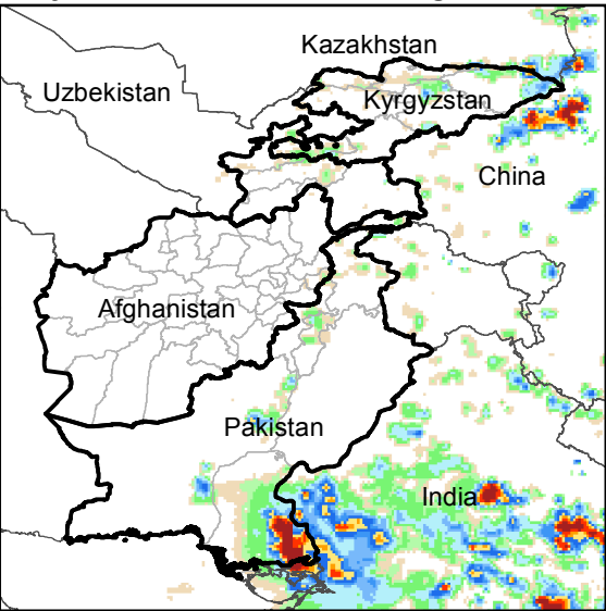
Daily Rainfall estimate for 26 Aug., 2016
