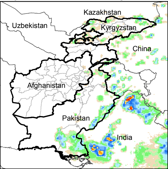
Daily Rainfall estimate for 25 Aug., 2016
