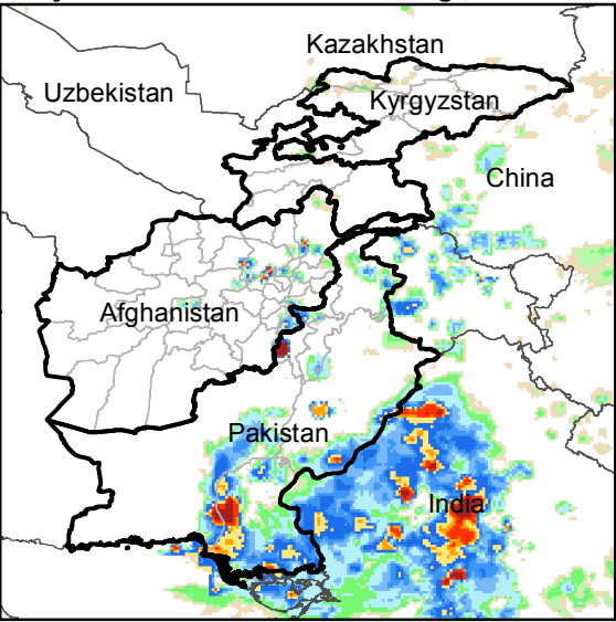
Daily Rainfall estimate for 28 Aug., 2016
