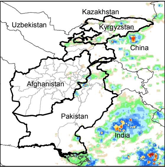
Daily Rainfall estimate for 29 Aug., 2016
