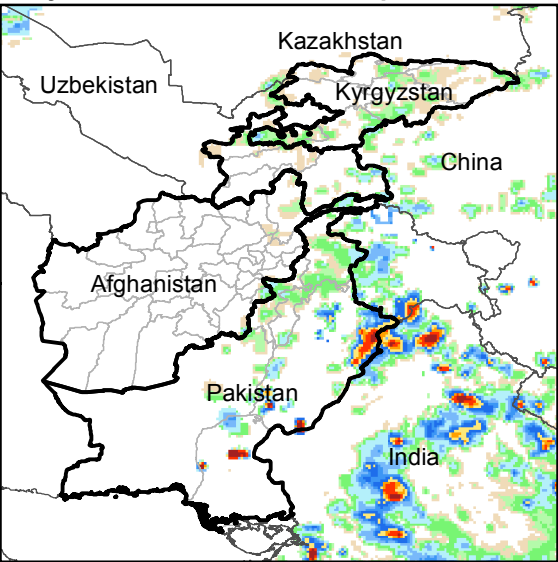
Daily Rainfall estimate for 4 Sep., 2016
