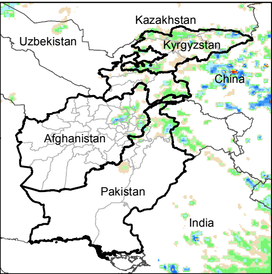
Daily Rainfall estimate for 5 Sep., 2016
