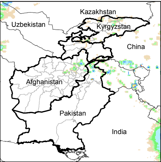
Daily Rainfall estimate for 10 Sep., 2016
