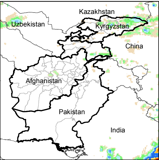
Daily Rainfall estimate for 28 Sep., 2016
