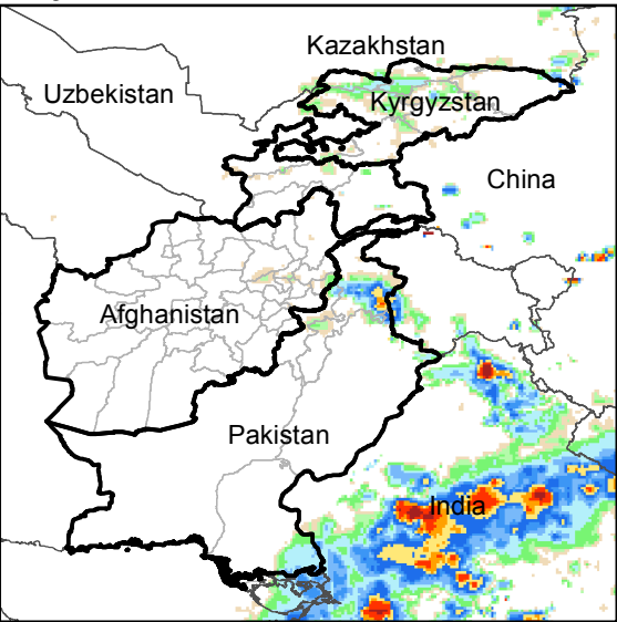
Daily Rainfall estimate for 8 Oct., 2016
