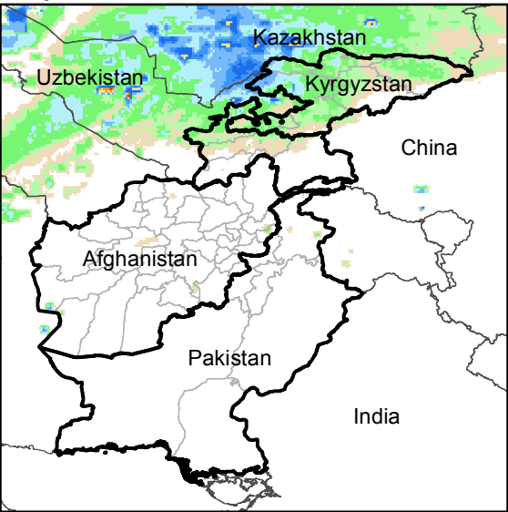
Daily Rainfall estimate for 10 Dec., 2016
