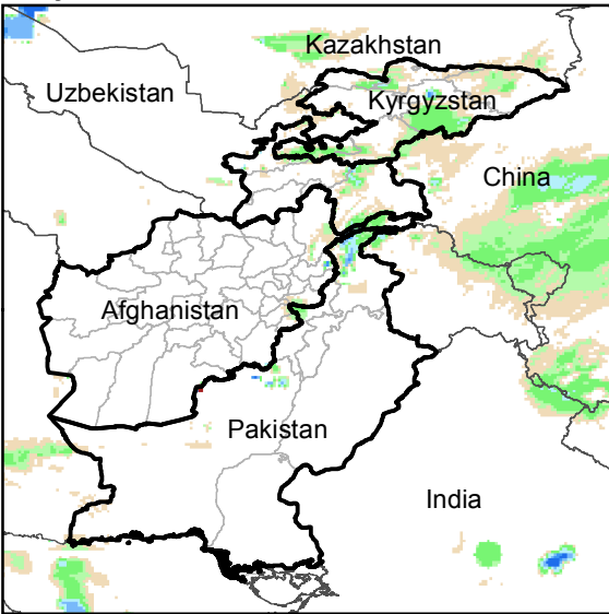
Daily Rainfall estimate for 22 Jan., 2017
