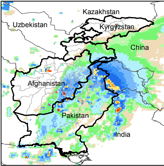
Daily Rainfall estimate for 25 Jan., 2017
