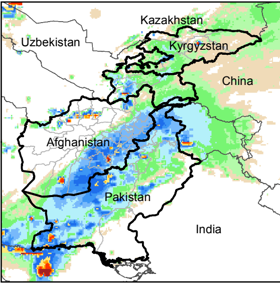
Daily Rainfall estimate for 24 Jan., 2017
