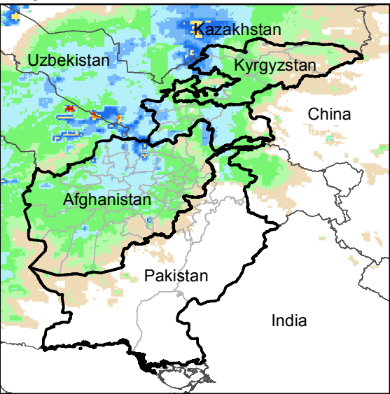
Daily Rainfall estimate for 14 Feb., 2017
