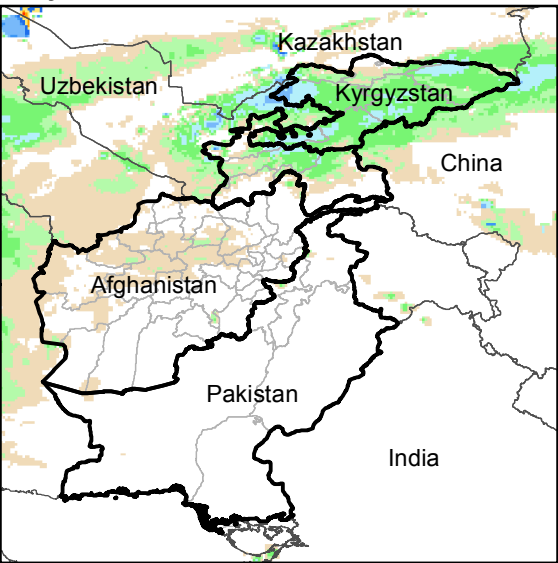
Daily Rainfall estimate for 13 Feb., 2017
