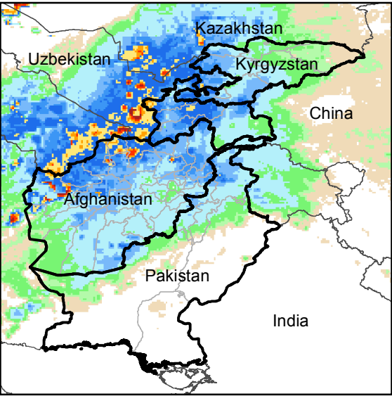
Daily Rainfall estimate for 18 Feb., 2017
