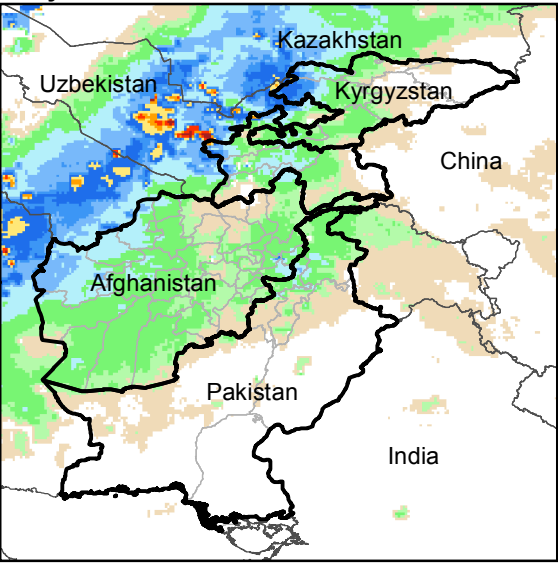
Daily Rainfall estimate for 17 Feb., 2017
