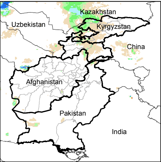
Daily Rainfall estimate for 27 Feb., 2017
