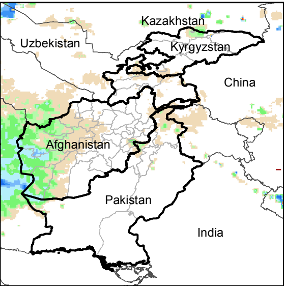
Daily Rainfall estimate for 23 Mar., 2017
