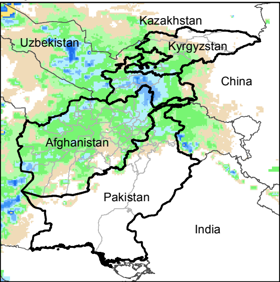
Daily Rainfall estimate for 24 Mar., 2017
