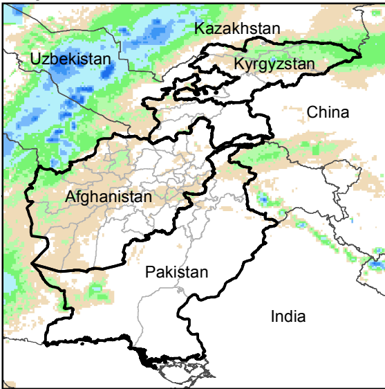
Daily Rainfall estimate for 28 Mar., 2017
