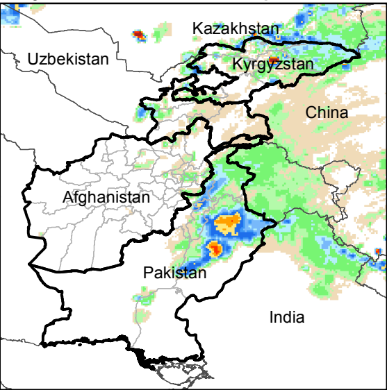
Daily Rainfall estimate for 25 Apr., 2017
