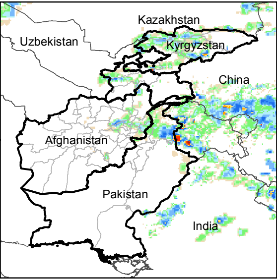
Daily Rainfall estimate for 24 Apr., 2017
