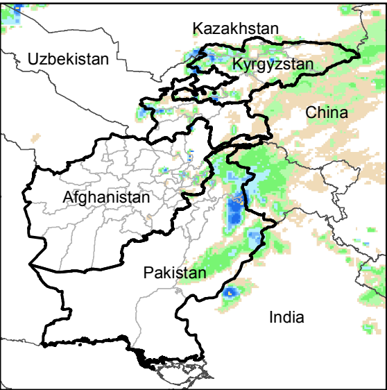
Daily Rainfall estimate for 26 Apr., 2017
