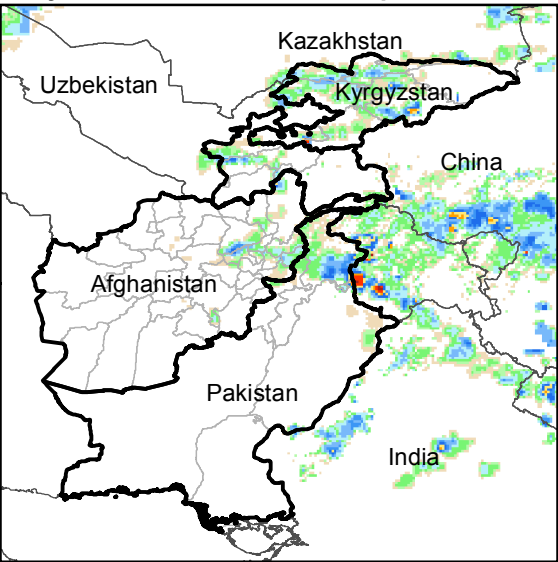
Daily Rainfall estimate for 27 Apr., 2017
