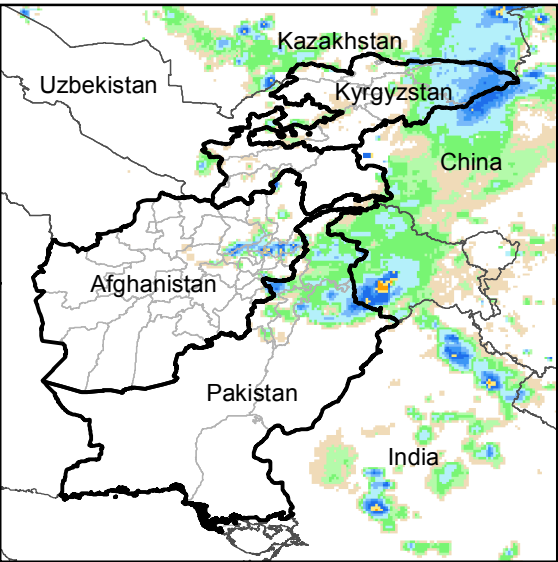
Daily Rainfall estimate for 2 May., 2017
