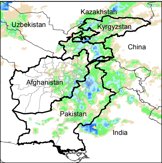
Daily Rainfall estimate for 19 May., 2017
