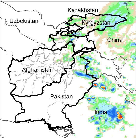
Daily Rainfall estimate for 3 Jun., 2017
