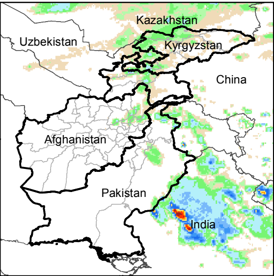
Daily Rainfall estimate for 1 Jun., 2017
