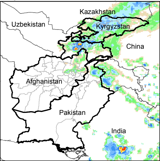
Daily Rainfall estimate for 2 Jun., 2017
