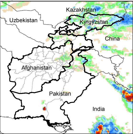
Daily Rainfall estimate for 8 Jun., 2017
