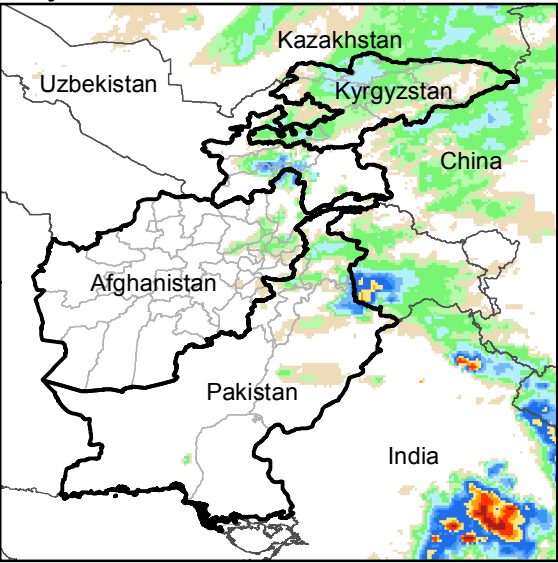
Daily Rainfall estimate for 6 Jun., 2017
