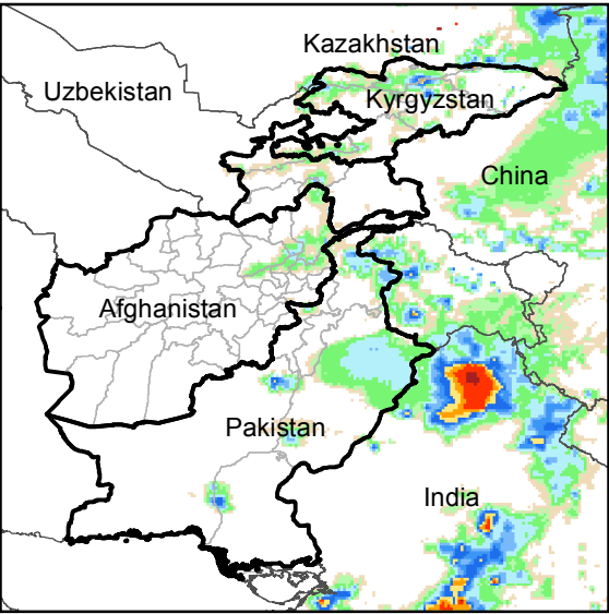
Daily Rainfall estimate for 7 Jun., 2017
