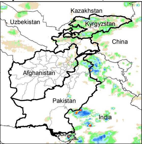
Daily Rainfall estimate for 9 Jun., 2017
